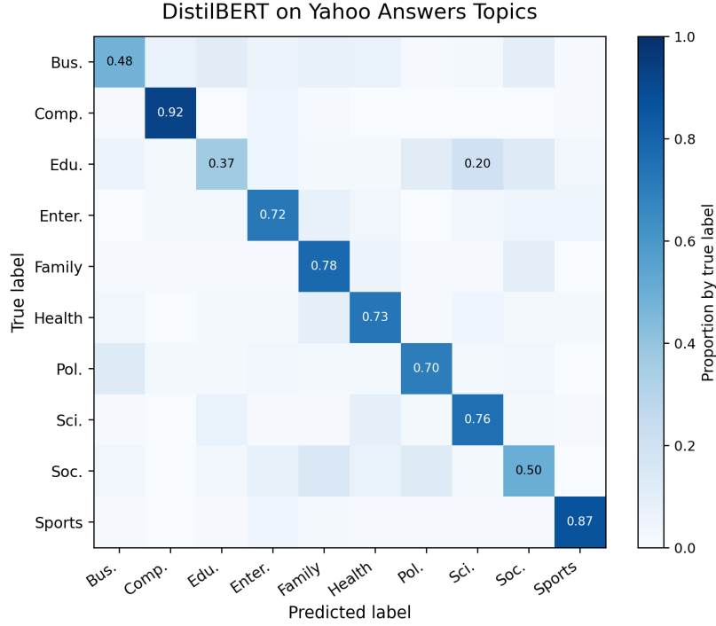
(a) DistilBERT
