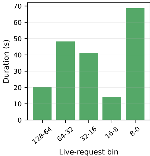
DeepSeek R1 7B CoT Lifetime, bs128, temp=0.9, 32K cap (drain 192s, p50 2212, p99 17636)
