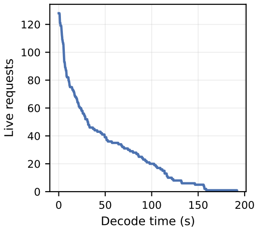
DeepSeek R1 7B CoT Lifetime, bs128, temp=0.9, 32K cap (drain 192s, p50 2212, p99 17636)
