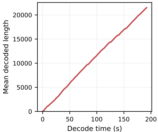
DeepSeek R1 7B CoT Lifetime, bs128, temp=0.9, 32K cap (drain 192s, p50 2212, p99 17636)
