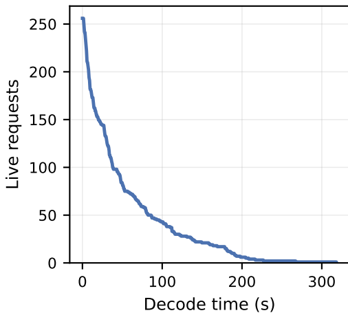
DeepSeek R1 7B CoT Lifetime, bs256, temp=0.9, 32K cap (drain 319s, p50 2199, p99 22734)
