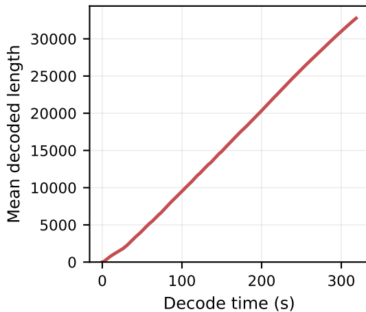
DeepSeek R1 7B CoT Lifetime, bs256, temp=0.9, 32K cap (drain 319s, p50 2199, p99 22734)
