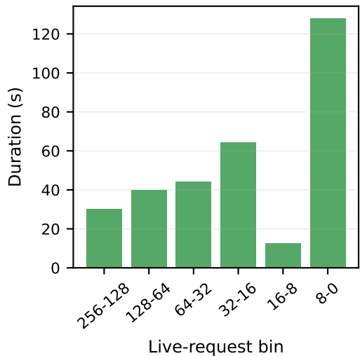
DeepSeek R1 7B CoT Lifetime, bs256, temp=0.9, 32K cap (drain 319s, p50 2199, p99 22734)
