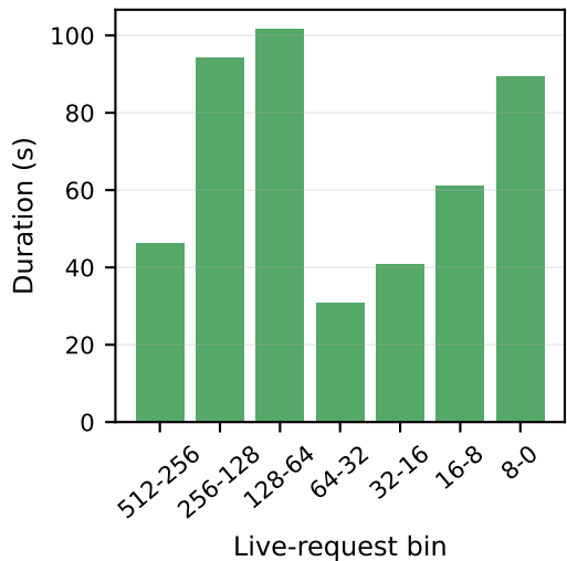
DeepSeek R1 7B CoT Lifetime, bs512, temp=0.9, 32K cap (drain 465s, p50 2074, p99 29364)
