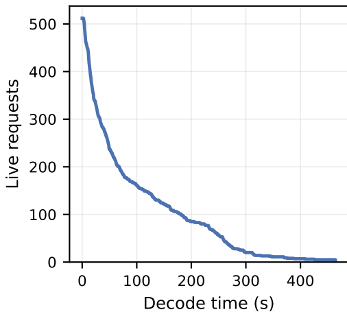
DeepSeek R1 7B CoT Lifetime, bs512, temp=0.9, 32K cap (drain 465s, p50 2074, p99 29364)
