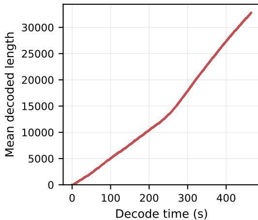
DeepSeek R1 7B CoT Lifetime, bs512, temp=0.9, 32K cap (drain 465s, p50 2074, p99 29364)
