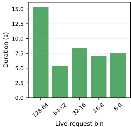
Qwen2.5-14B-Instruct on Eurús-2-RL, TP1, bs128, temp=0.9, 32K cap (drain 44s, p50 371, p99 1455)
