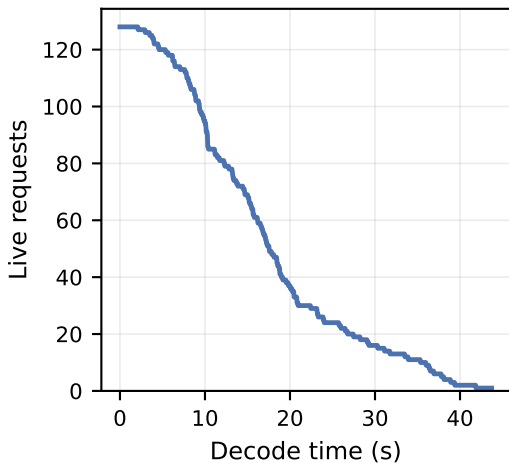
Qwen2.5-14B-Instruct on Eurús-2-RL, TP1, bs128, temp=0.9, 32K cap (drain 44s, p50 371, p99 1455)
