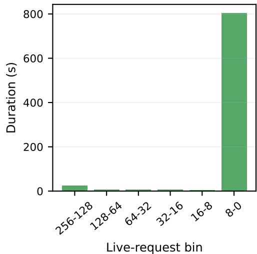
Qwen2.5-14B-Instruct on Euror-2-RL, TP1, bs256, temp=0.9, 32K cap (drain 850s, p50 326, p99 1548)
