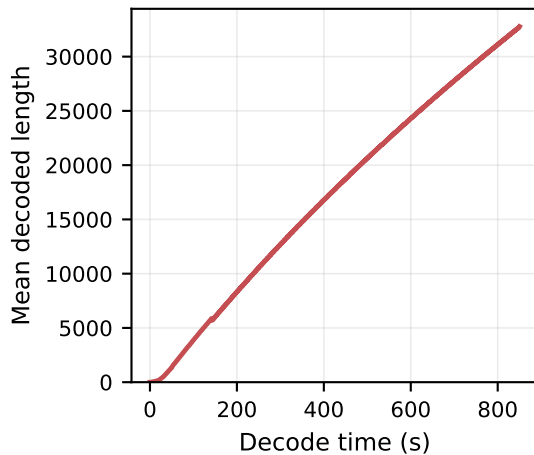
Qwen2.5-14B-Instruct on Euror-2-RL, TP1, bs256, temp=0.9, 32K cap (drain 850s, p50 326, p99 1548)
