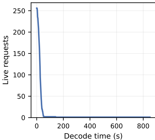
Qwen2.5-14B-Instruct on Euror-2-RL, TP1, bs256, temp=0.9, 32K cap (drain 850s, p50 326, p99 1548)
