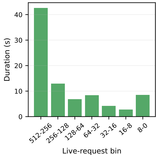
Qwen2.5-14B-Instruct on Euror-2-RL, TP1, bs512, temp=0.9, 32K cap (drain 86s, p50 329, p99 1631)
