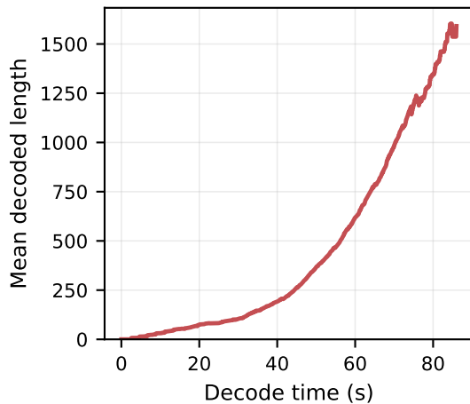
Qwen2.5-14B-Instruct on Euror-2-RL, TP1, bs512, temp=0.9, 32K cap (drain 86s, p50 329, p99 1631)
