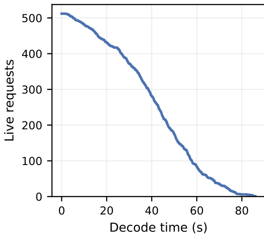
Qwen2.5-14B-Instruct on Euror-2-RL, TP1, bs512, temp=0.9, 32K cap (drain 86s, p50 329, p99 1631)
