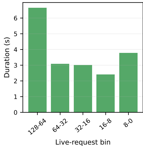
Qwen2.5-14B-Instruct on Euror-2-RL, TP4, bs128, temp=0.9, 32K cap (drain 19s, p50 406, p99 1564)
