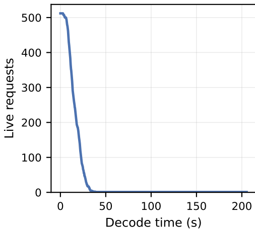
Qwen2.5-14B-Instruct on Eurur-2-RL, TP4, bs512, temp=0.9, 32K cap (drain 205s, p50 344, p99 1617)
