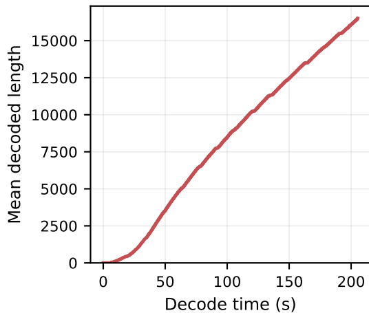
Qwen2.5-14B-Instruct on Eurur-2-RL, TP4, bs512, temp=0.9, 32K cap (drain 205s, p50 344, p99 1617)
