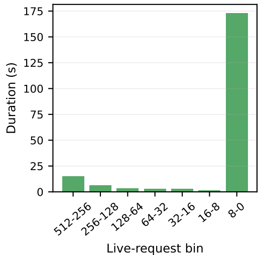
Qwen2.5-14B-Instruct on Eurur-2-RL, TP4, bs512, temp=0.9, 32K cap (drain 205s, p50 344, p99 1617)
