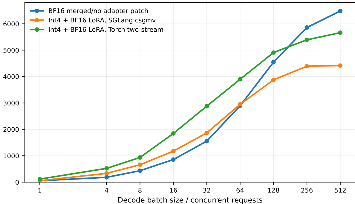
QLoRA Rollout Decoding Throughput
