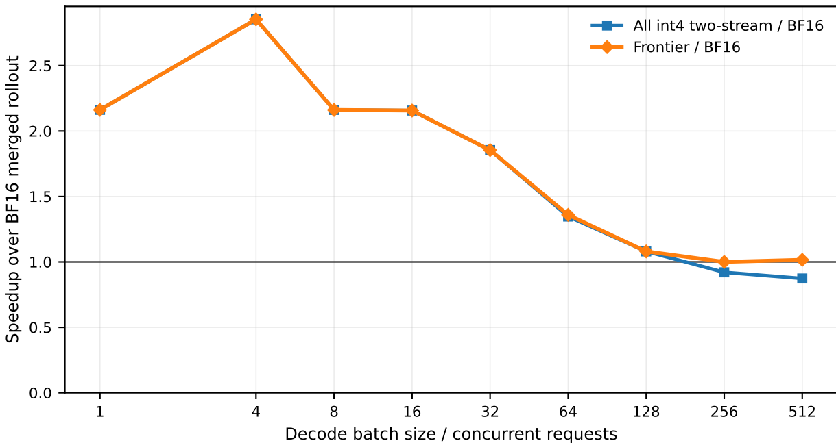
Kernel-Guided Decode Speedup (qwen2.5-14b)
