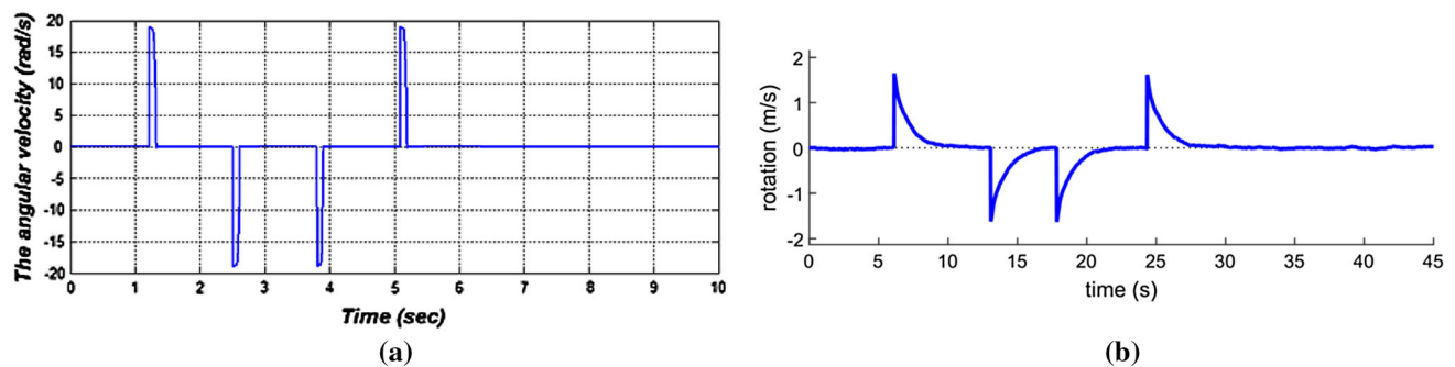
Fig. 24 The robot angular velocity of tracking a pulse trajectory: a the proposed approach and b the approach of Wang et al. (2018b)
