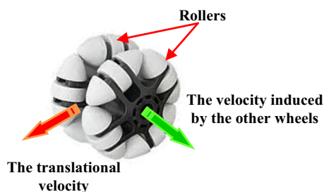
Fig. 2 The omni-wheel
