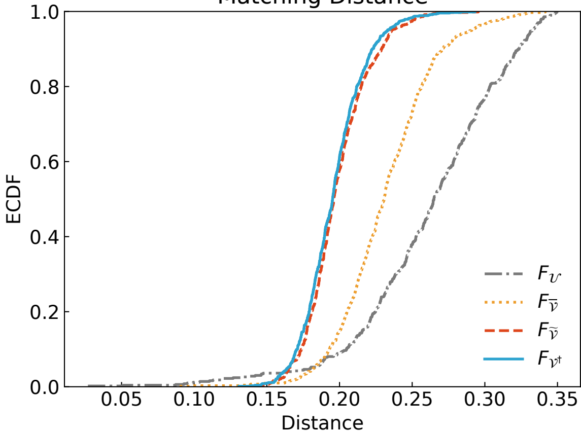
Plot C: Empirical CDF on Prediction_b (shared samples)
