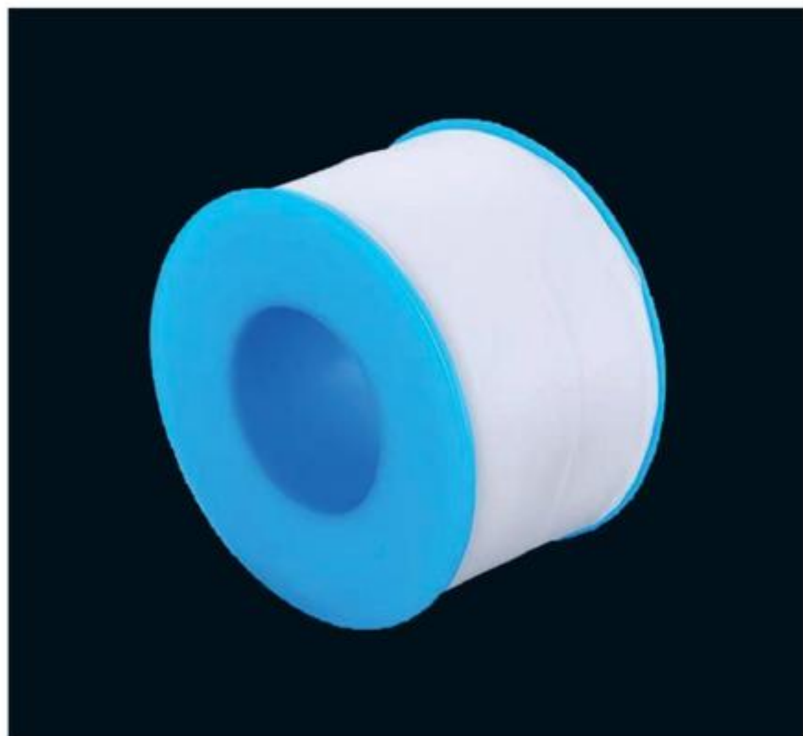
产品型号 (ITEM NO.): JC-11 WIDTH:48MM LENGTH:30-50M DENSITY:0.25G/CM3-1.0G/CM3 THICKNESS:0,1MM-0.2mm
