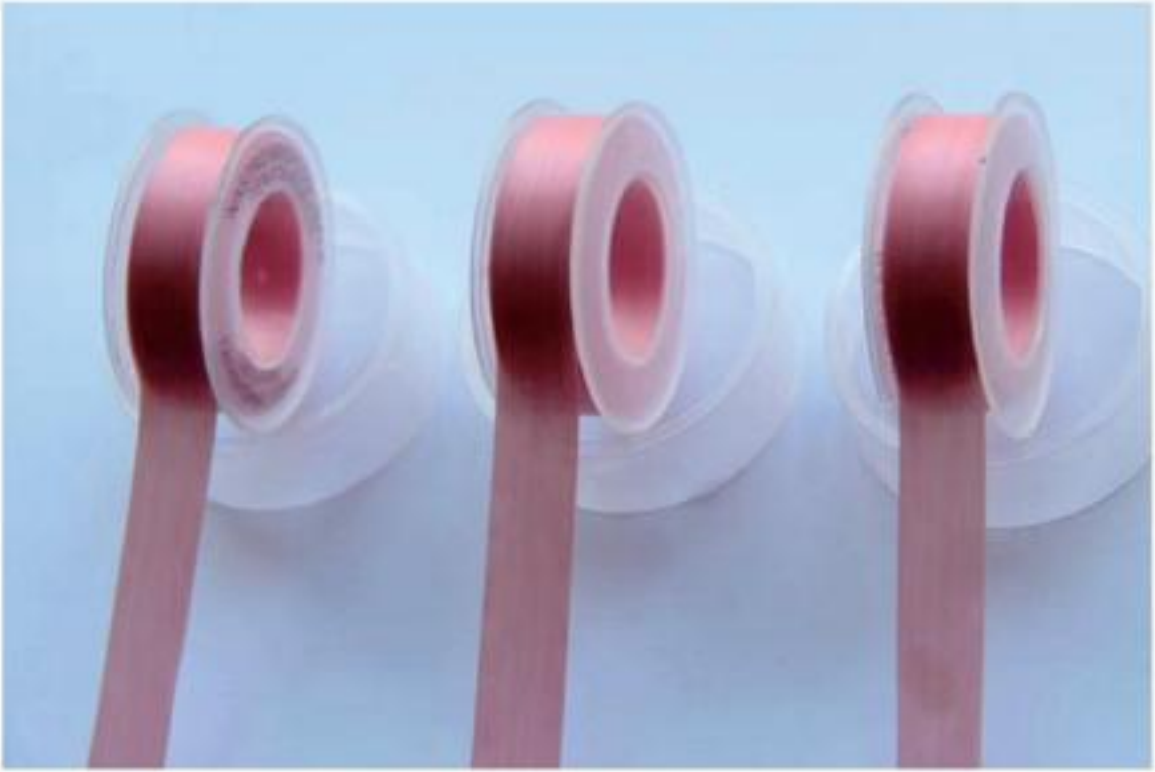
产品型号 (ITEM NO.): JC-18 PINK TAPE WIDTH:12MM LENGTH:10-15M DENSITY :0.25G/CM3-1.0G/CM3 THICKNESS :0.075MM-0,1MM
