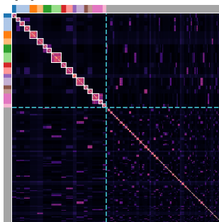
(b) Full-code MSE
