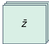
Target code
