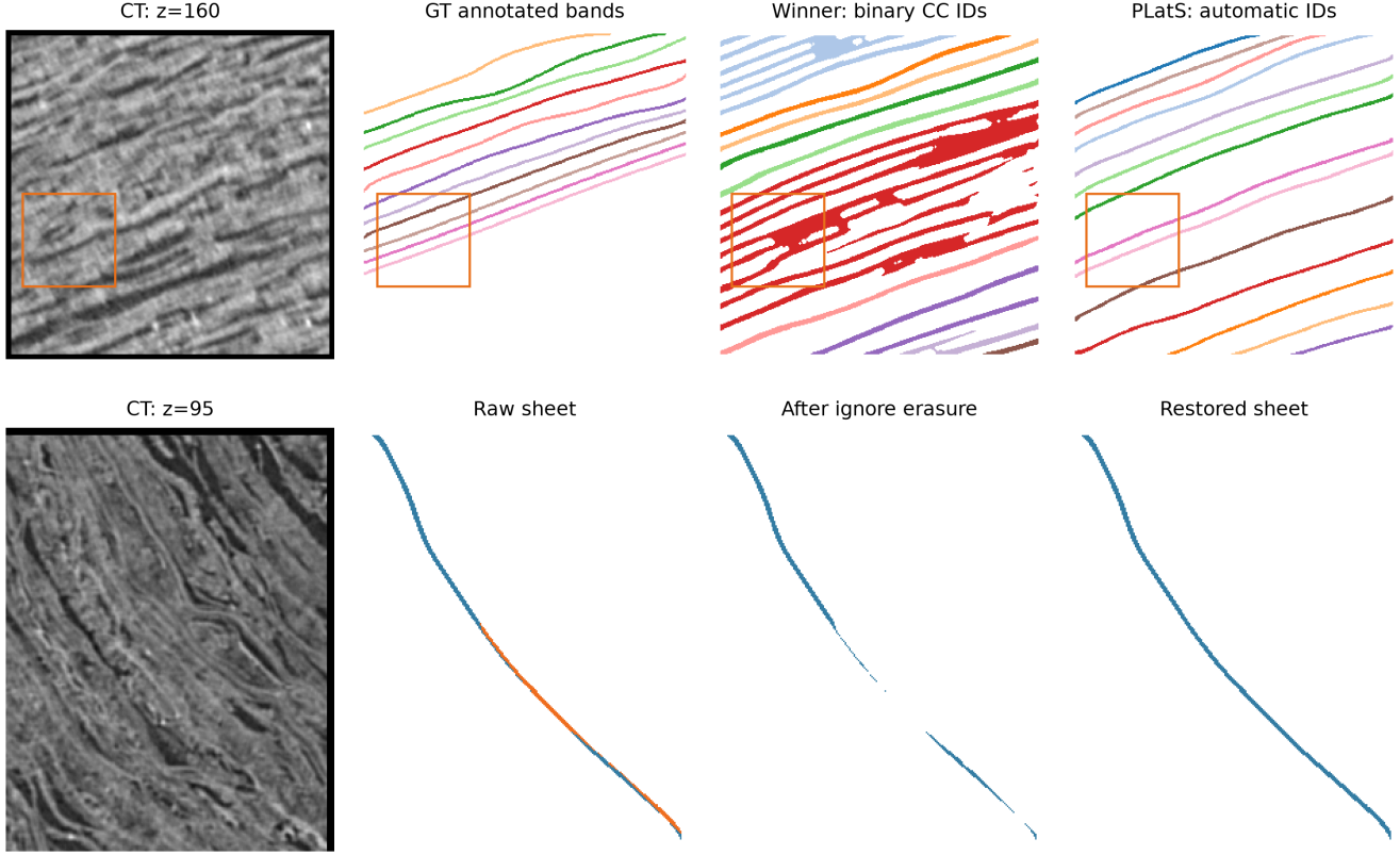
Figure 4. Two different topology failures. Top: a winner component joins six annotated bands in case 00860 ( z = 160 ); Base PLaTS preserves gaps but misses bands. Colors are IDs within each method. Bottom: ignore erasure cuts a predicted sheet in case 00829 ( z = 95 ). Its whole-volume topology changes from one component and no tunnels to 495 components and 1,023 tunnels. Restoring its own voxels reverses the cuts. Orange marks removed voxels. Both rows use native z slices; selection rules and the enlarged orange-square crop are in Supplementary.
