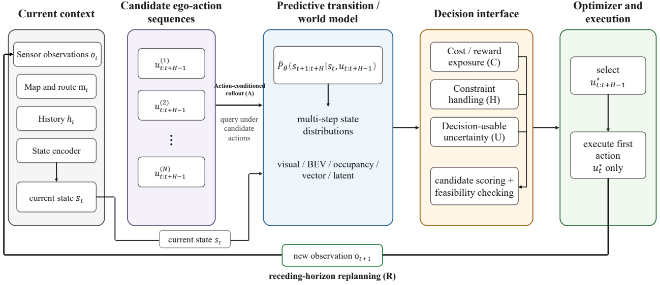
Fig. 2. Representative MPC-oriented information flow for a driving world model. Candidate ego-action sequences query a predictive transition; multi-step state distributions expose costs or rewards, constraints, and decision-usable uncertainty; the optimizer executes only the first selected action before replanning from the next observation. The family overlays indicate where reviewed methods enter the loop rather than asserting that every method implements all five MPC interface elements.
