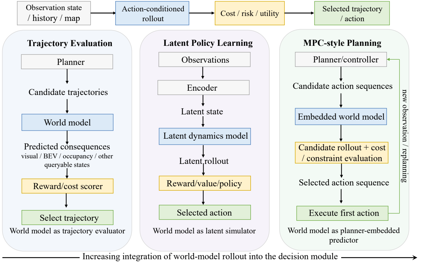
Fig. 5. Planning with world models. Imagined futures are consumed through a separable decision interface for trajectory evaluation, latent policy learning, or MPC-style rollout rather than treated as standalone generated samples. These subclasses are distinguished by how the rollouts enter the decision module, not by whether the predicted state is visual, BEV, occupancy, vector, or latent.
