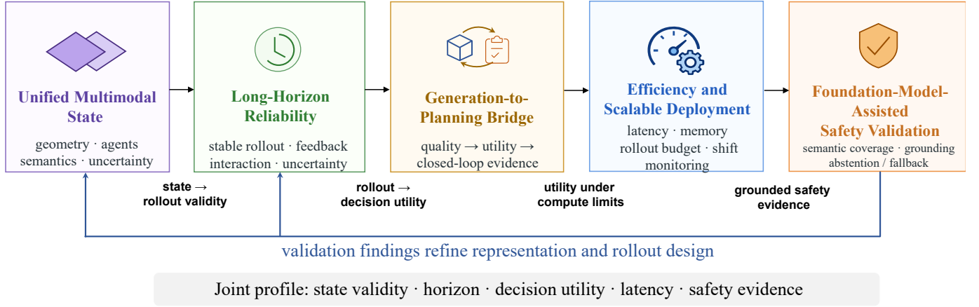
Fig. 7. MPC-oriented future challenges for autonomous-driving world models. The five directions form a dependency chain from unified multimodal state and reliable long-horizon rollout to decision utility, scalable deployment, and grounded safety evidence. Validation findings feed back to representation and rollout design, and progress should be reported as a joint profile of state validity, horizon, decision utility, latency, and safety evidence.
