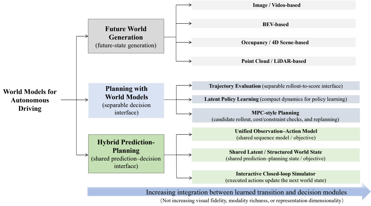
Fig. 3. A task-oriented taxonomy of autonomous-driving world models based on each method’s primary task role: future world generation, planning with world models, or hybrid prediction–planning. The bottom arrow denotes increasing integration between learned transition and decision modules, not increasing visual fidelity, modality richness, or representation dimensionality.
