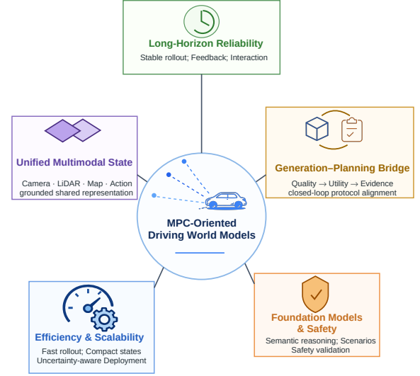
Fig. 7. MPC-oriented future challenges for autonomous-driving world models. The figure summarizes five connected directions: reliable long-horizon rollout, unified multimodal state representation, bridges from generation quality to planning utility and closed-loop evidence, efficient scalable deployment, and foundation-model-assisted safety validation.
