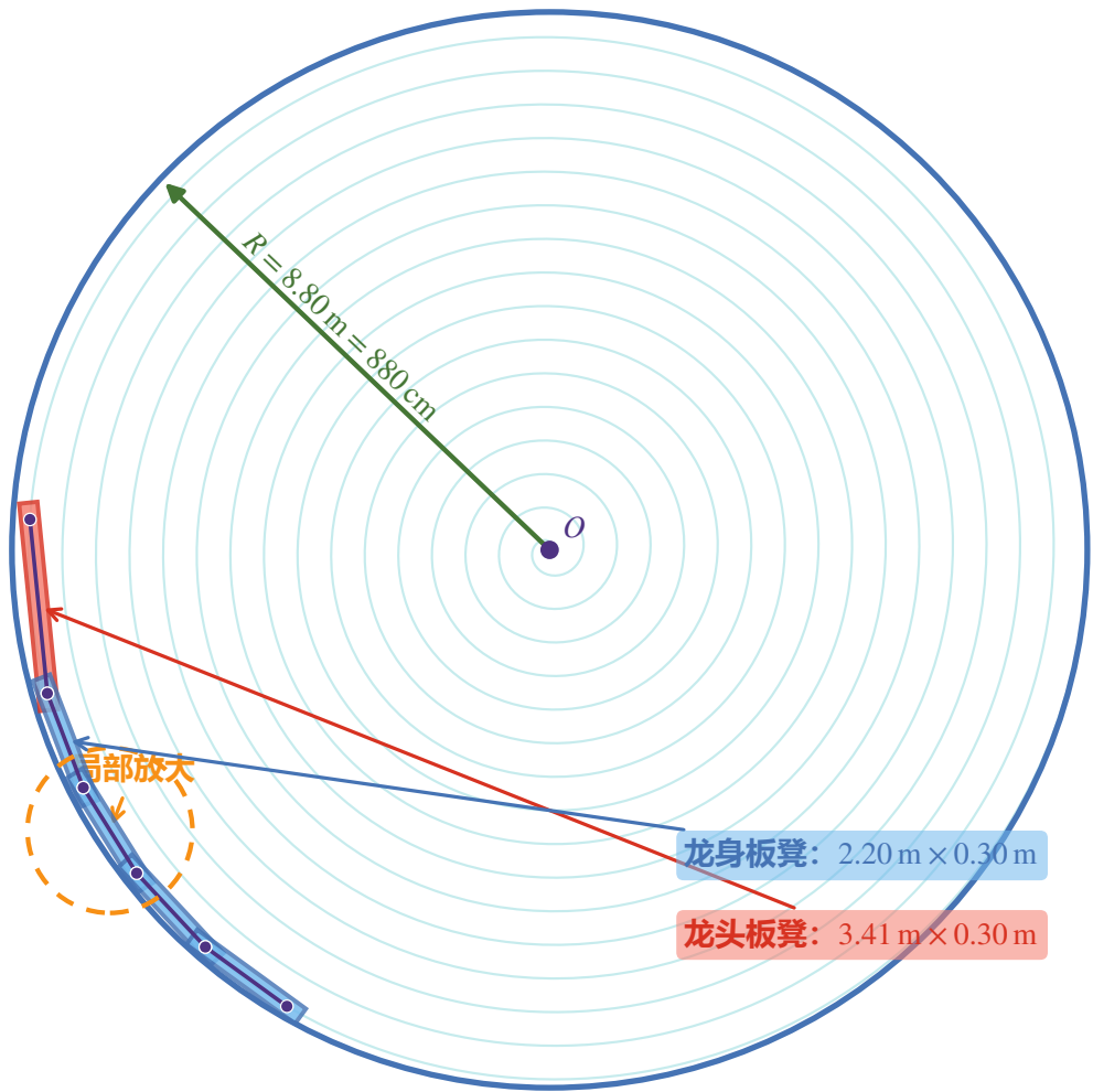
(a) R = 8.80\text{ m} (880 cm) 圆域内的板凳实体比例
