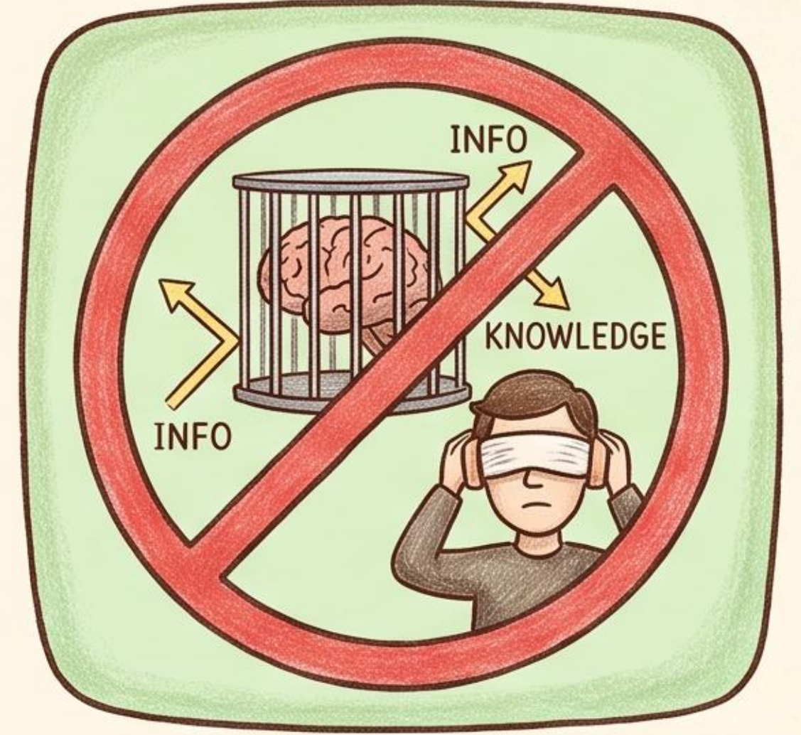
NO-LEARNING
