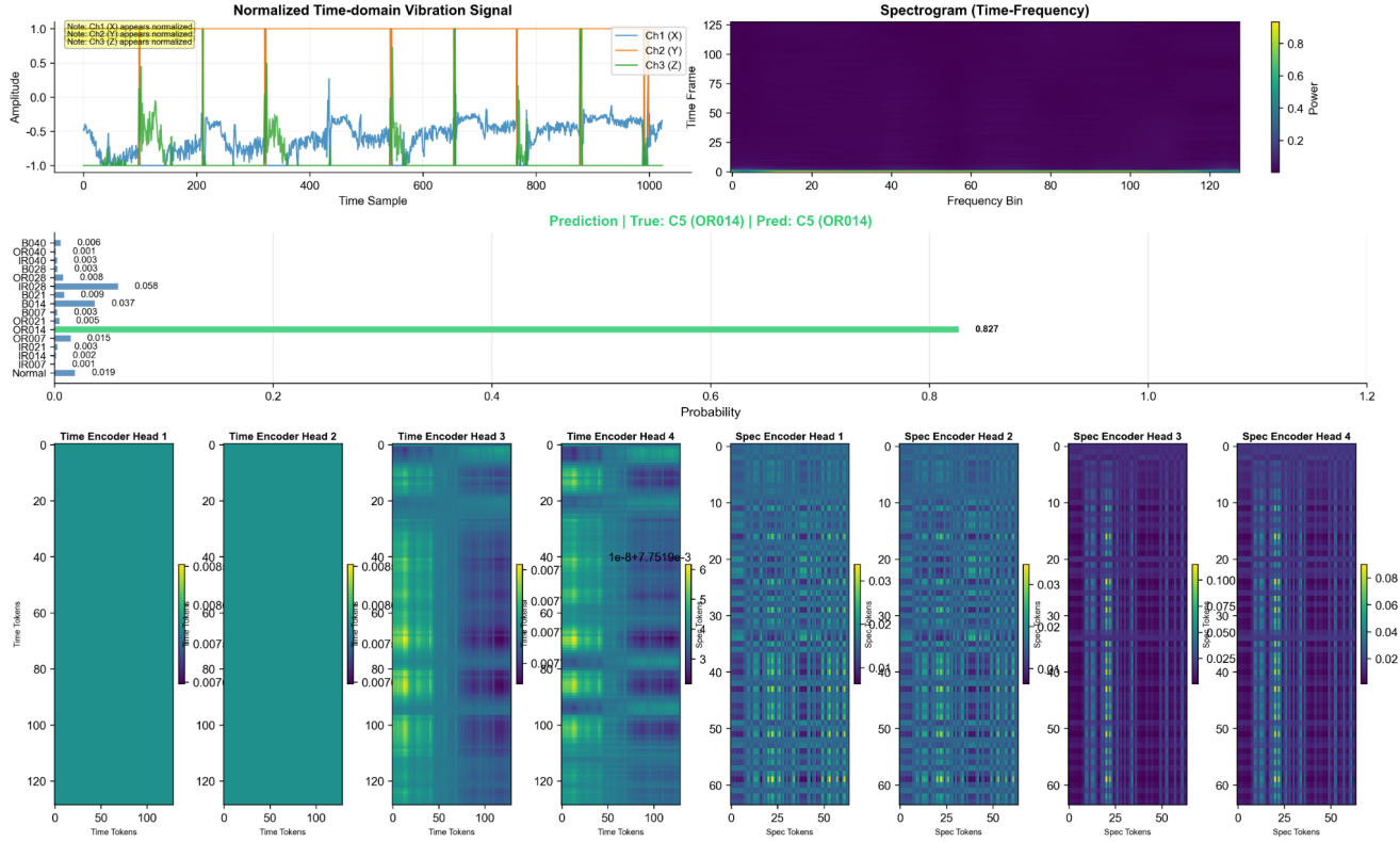
Fig. 7: Encoder self-attention visualization for a correctly classified C5 sample. The upper part shows the normalized three-channel vibration signal, spectrogram and prediction probability, while the lower part visualizes representative self-attention heads from the time-domain and spectrogram encoders.
