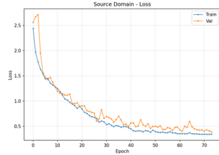
(a) Distill T=1.5, alpha=0.25
