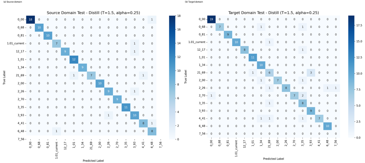
Fig. 4: Source-domain and target-domain confusion matrices of Distill ( T = 1.5 , \alpha = 0.25 ).
