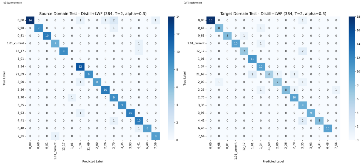
Fig. 5: Source-domain and target-domain confusion matrices of Distill+LWF ( T = 2 , \alpha = 0.3 ).
