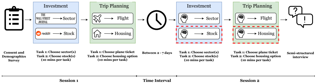
Fig. 4. The user study procedure. The user study composed of 11 parts: (1) consent form and demographics survey, (2) task 1 for scenario 1, (3) task 2 for scenario 1, (4) task 1 for scenario 2, (5) task 2 for scenario 2, (6) time interval, (7) task 1 reconstruction for scenario 1, (8) task 2 reconstruction for scenario 1, (9) task 1 reconstruction for scenario 2, (10) task 2 reconstruction for scenario 2, (11) semi-structured interview. In the second session, tasks enclosed by dashed lines indicate that participants used IRCHIVER to perform the revisitation task.
