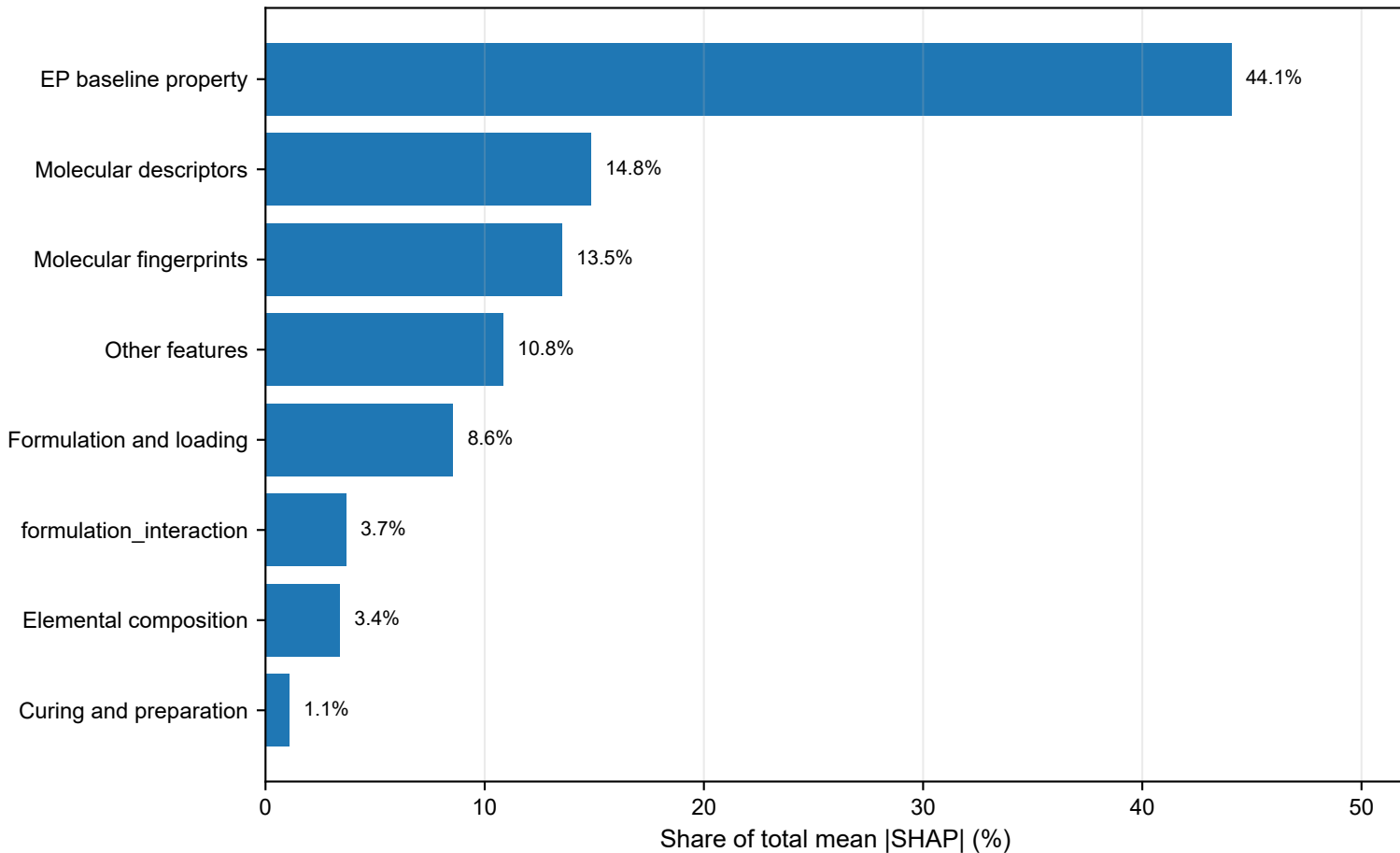
Tensile strength: SHAP contribution by feature group
