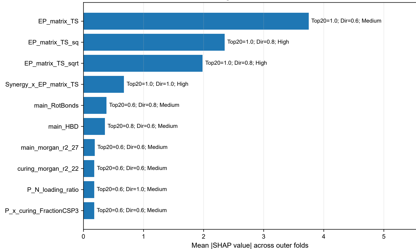
Tensile strength: stable SHAP features
