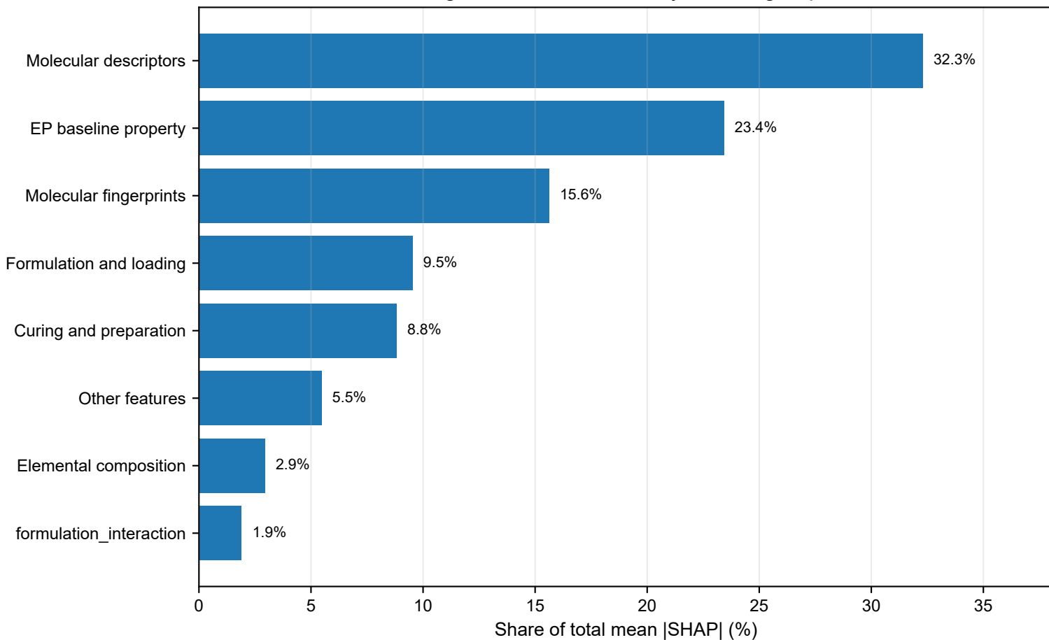
Tg: SHAP contribution by feature group
