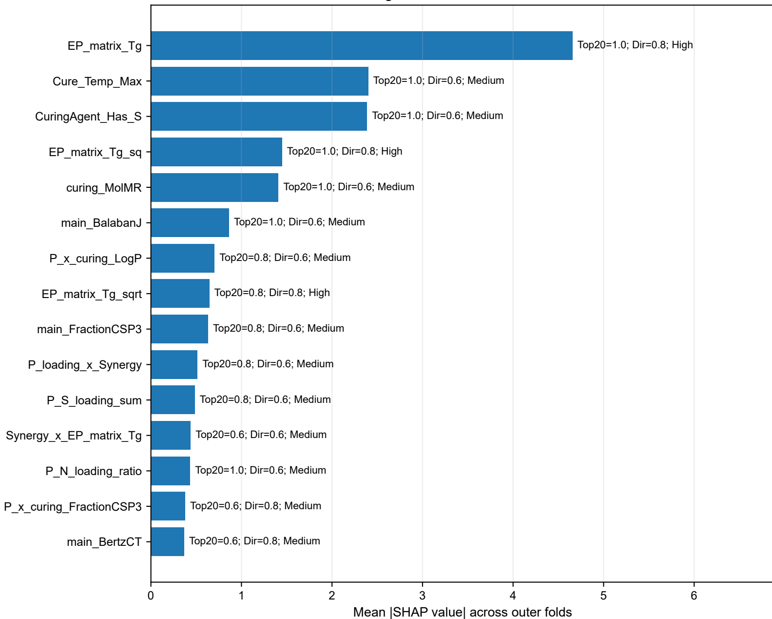
Tg: stable SHAP features
