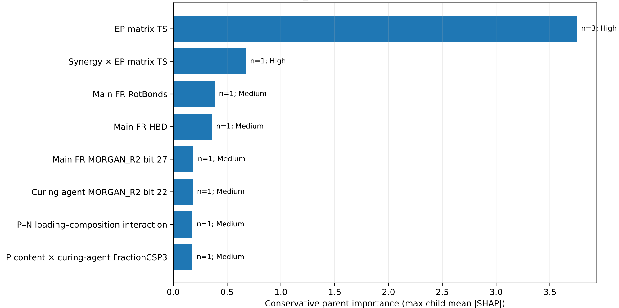
TS_MPa: stable SHAP parent variables
