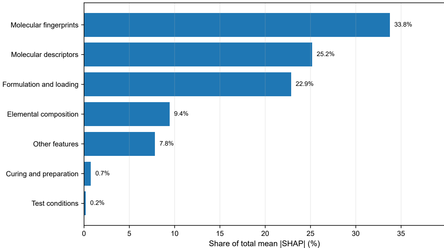
UL-94 V-0: SHAP contribution by feature group
