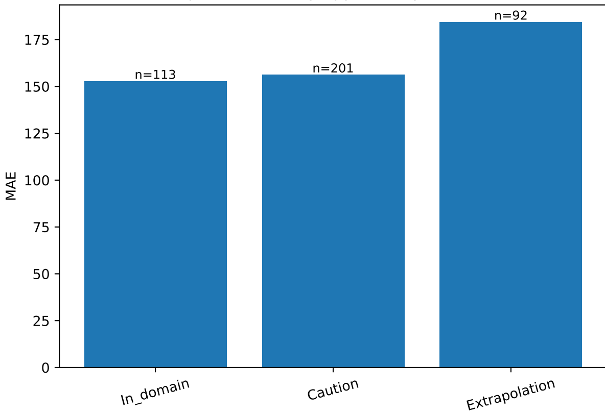
PHRR: performance by applicability-domain zone
