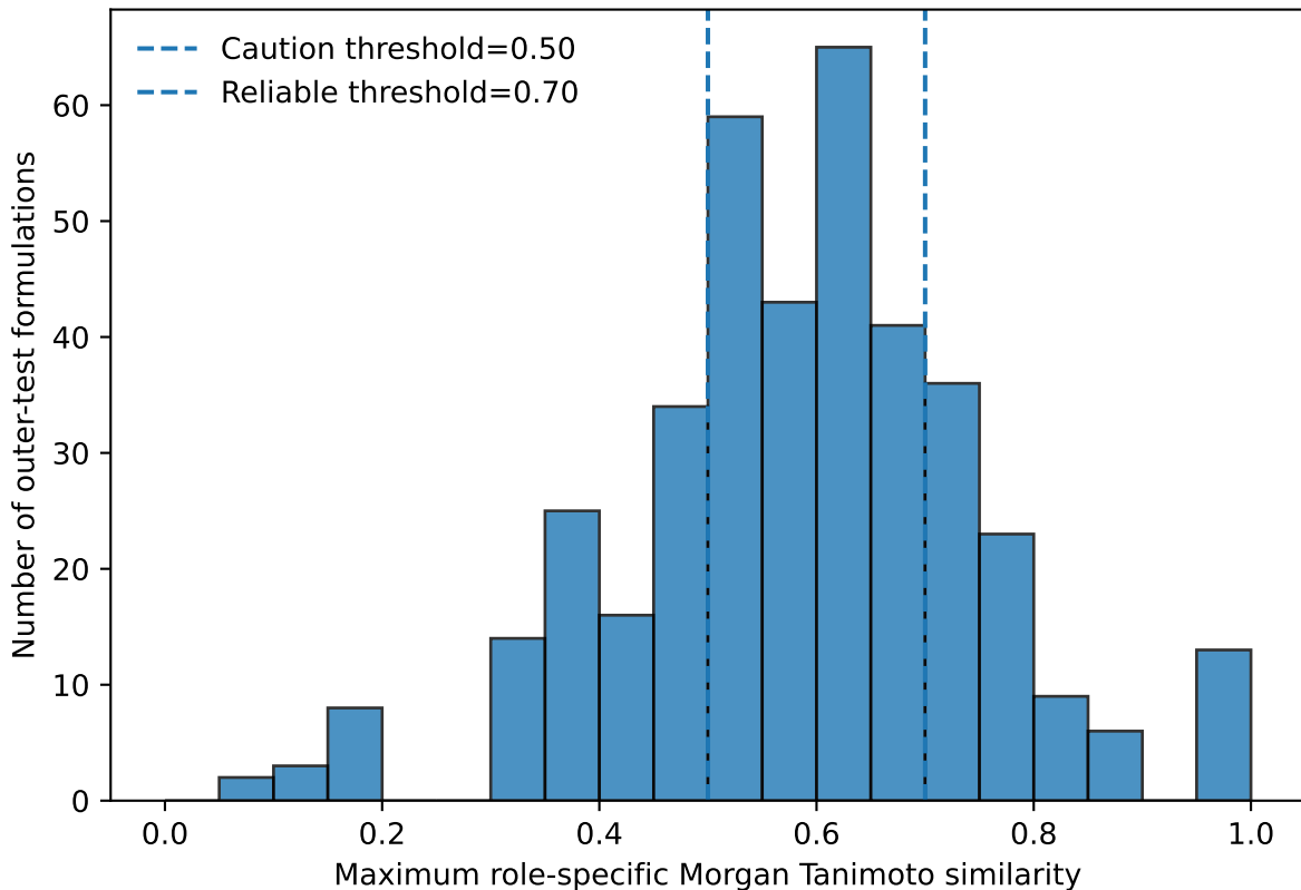
THR: structural-similarity distribution
