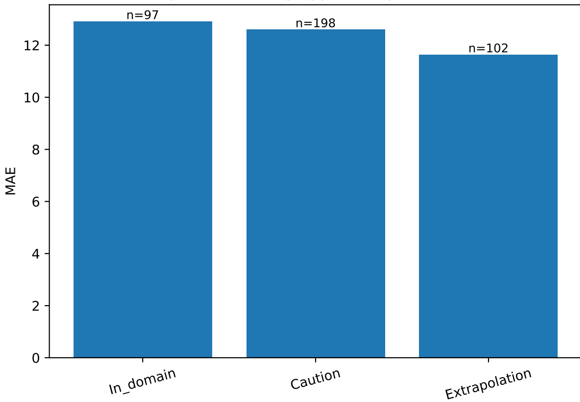
THR: performance by applicability-domain zone
