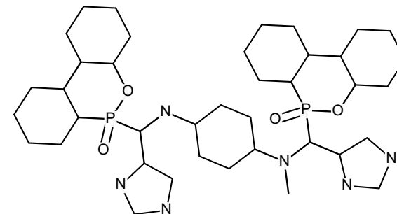
#9 DIB-NH-methyl P-N
