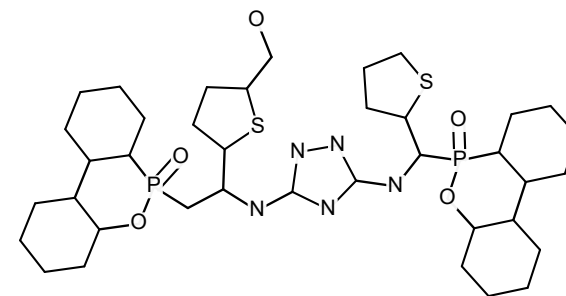
#4 BDO-hydroxymethyl P-N-S
