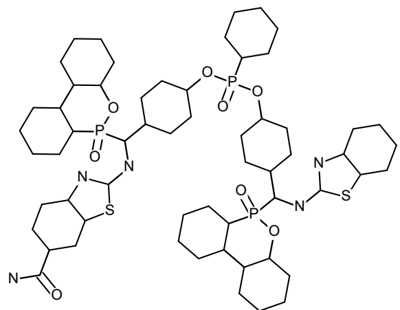
#7 PAD-carboxamide P-N-S
