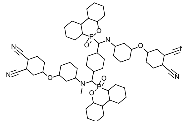
#5 PBD-NH-methyl P-N
