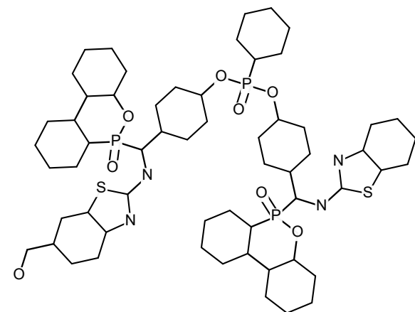
#10 PAD-hydroxymethyl P-N-S
