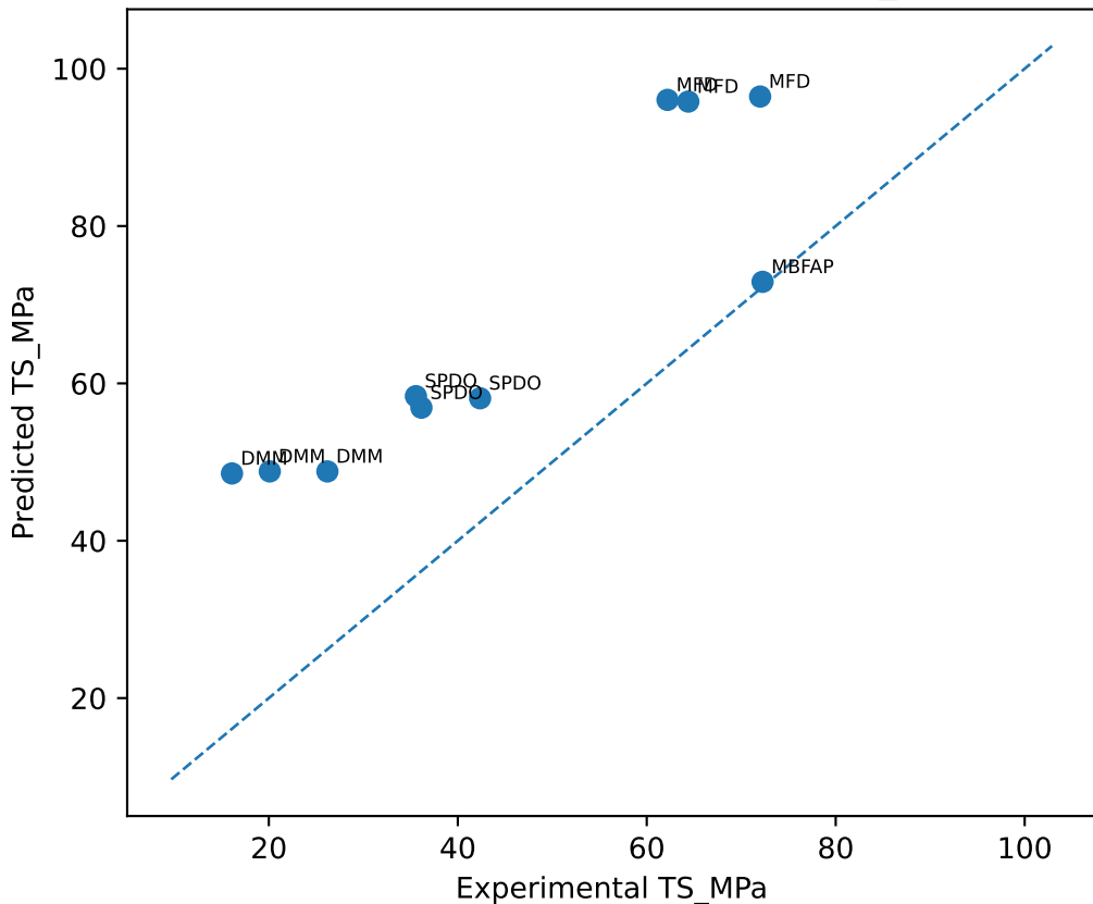
Independent external validation: TS_MPa
