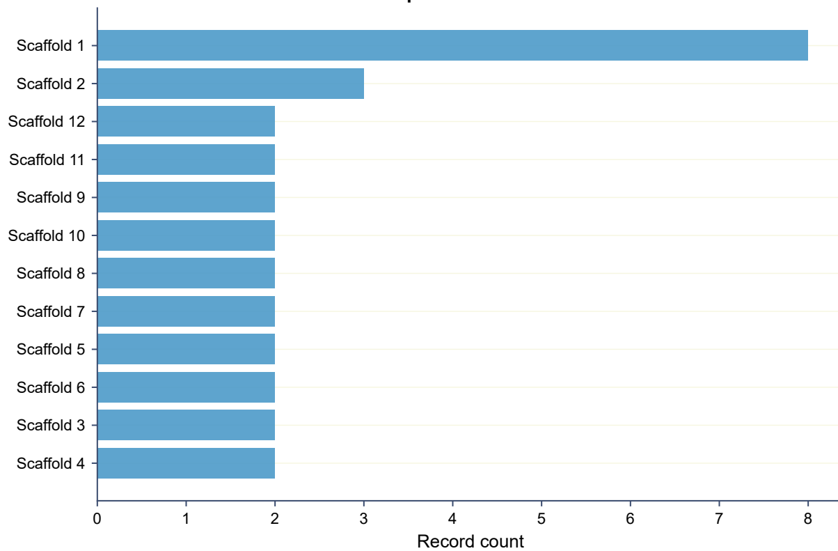
Most frequent Murcko scaffolds
