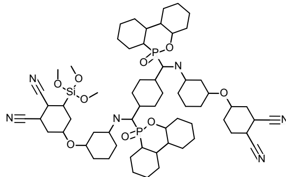
#2 PBD- trimethoxysilyl P-N-Si
