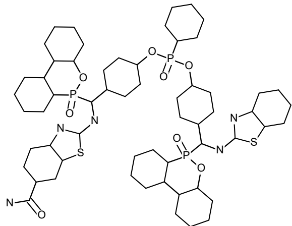
#7 PAD-carboxamide P-N-S
