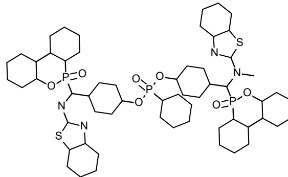
#3 PAD-NH-methyl P-N-S
