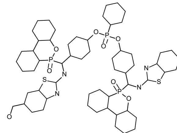
#10 PAD-hydroxymethyl P-N-S
