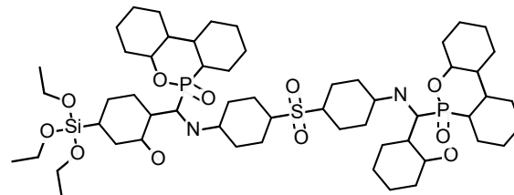
#8 DSD-triethoxysilyl P-N-Si-S
