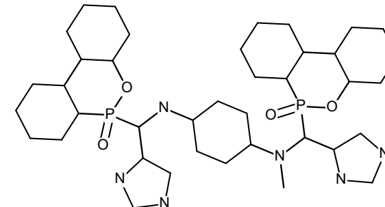
#9 DIB-NH-methyl P-N
