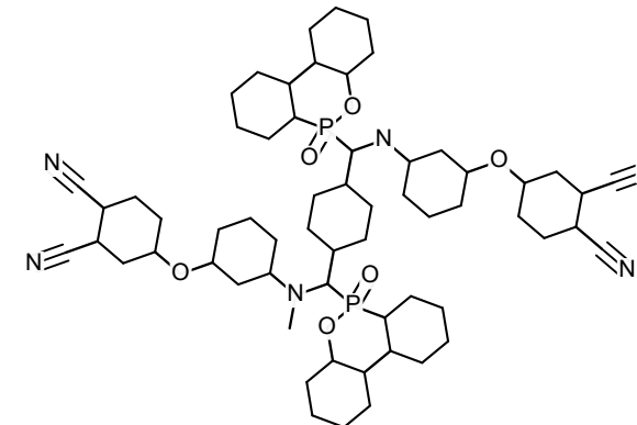
#5 PBD-NH-methyl P-N
