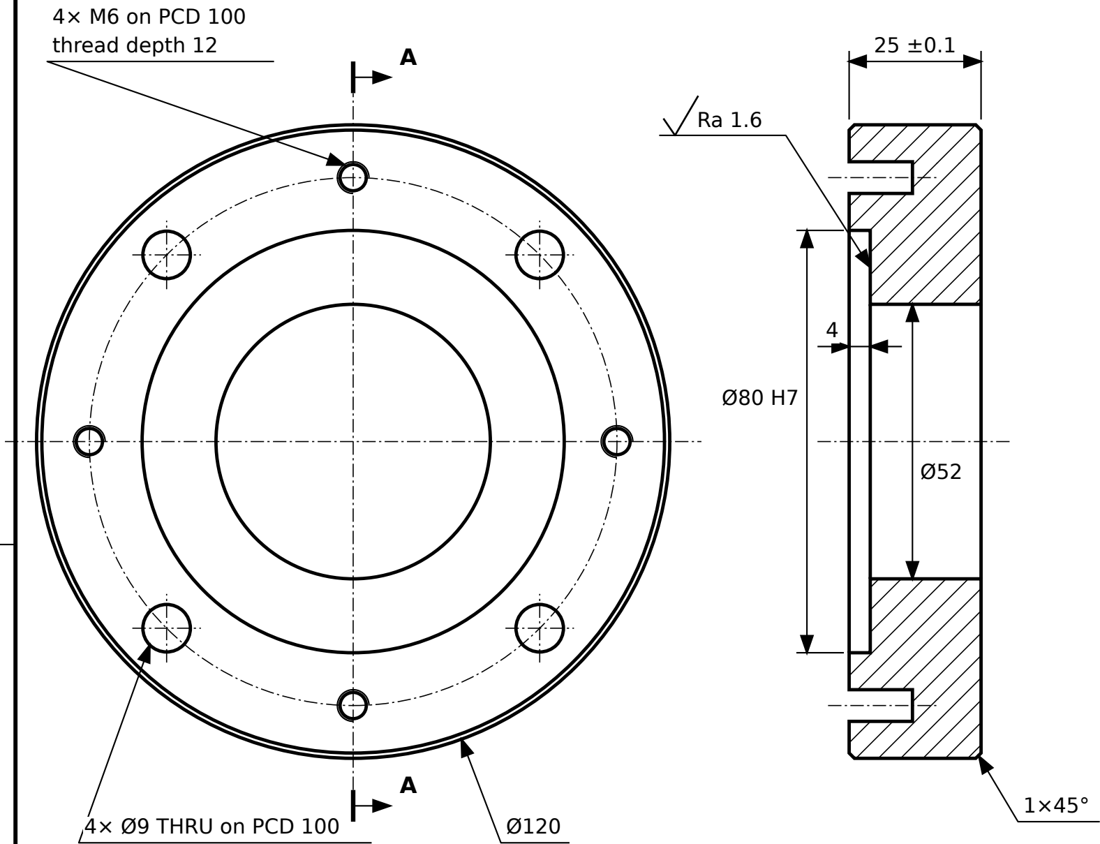
FRONT VIEW
