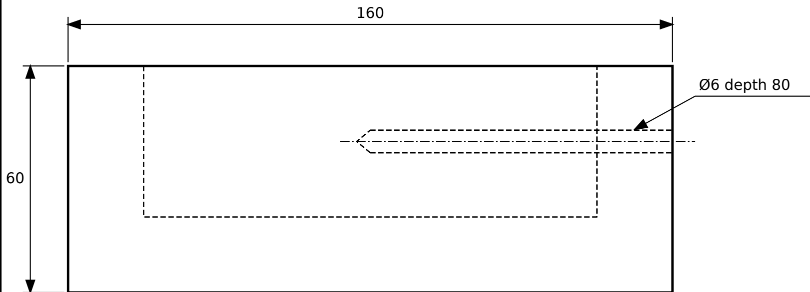
FRONT VIEW
