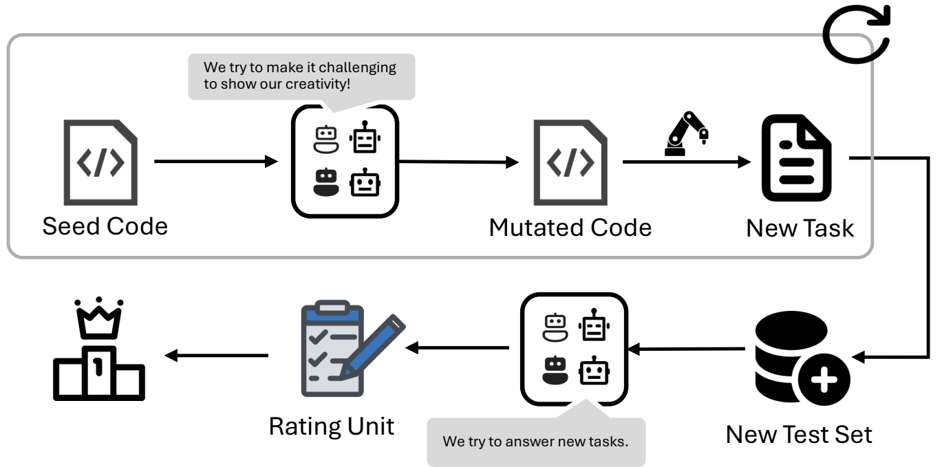
Figure 2: High-level workflow of CodeArena.
