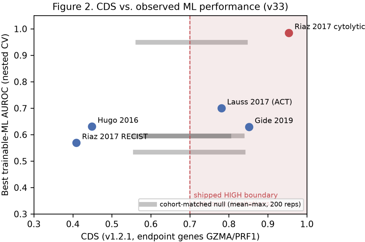
644 Figure S10. CDS vs observed ML performance (identical to main-text Figure 2)
