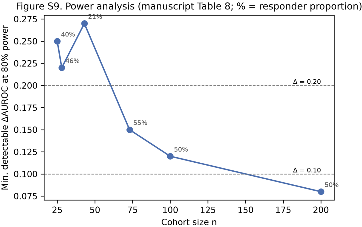
642 Figure S9. Power curves
