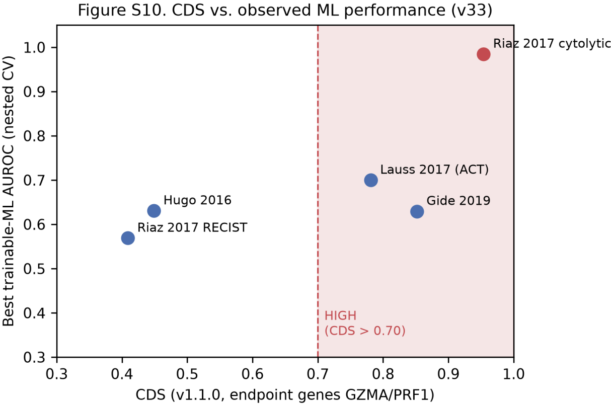
623 Figure S10. CDS vs observed ML performance (identical to main-text Figure 2)
