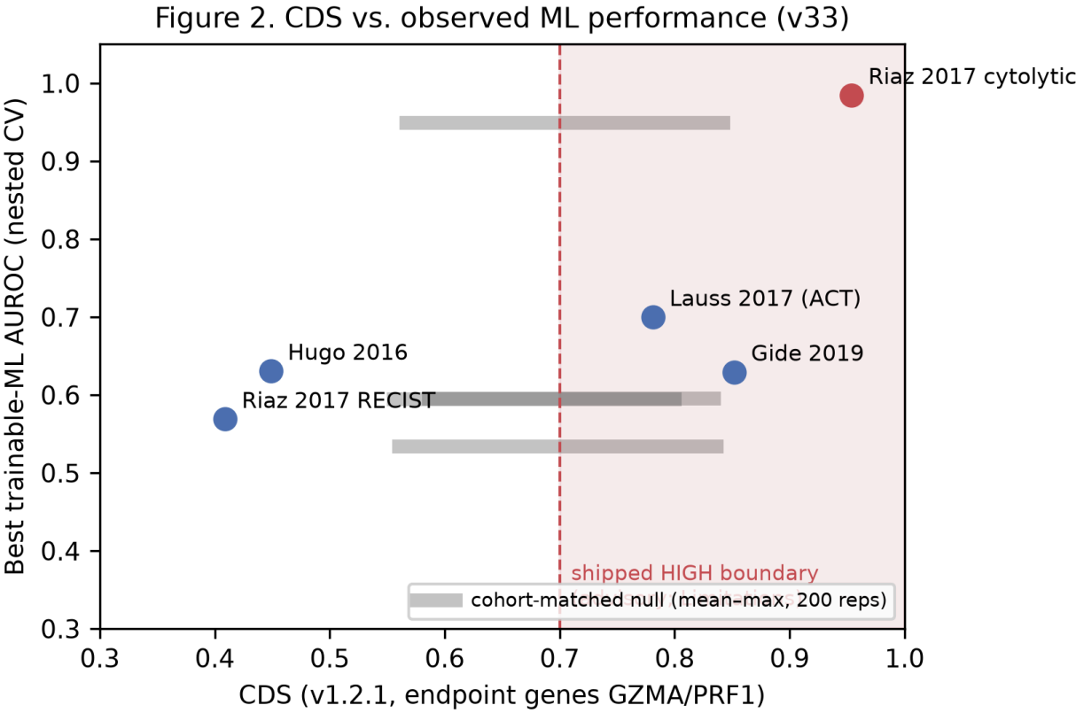
628 Figure S10. CDS vs observed ML performance (identical to main-text Figure 2)
