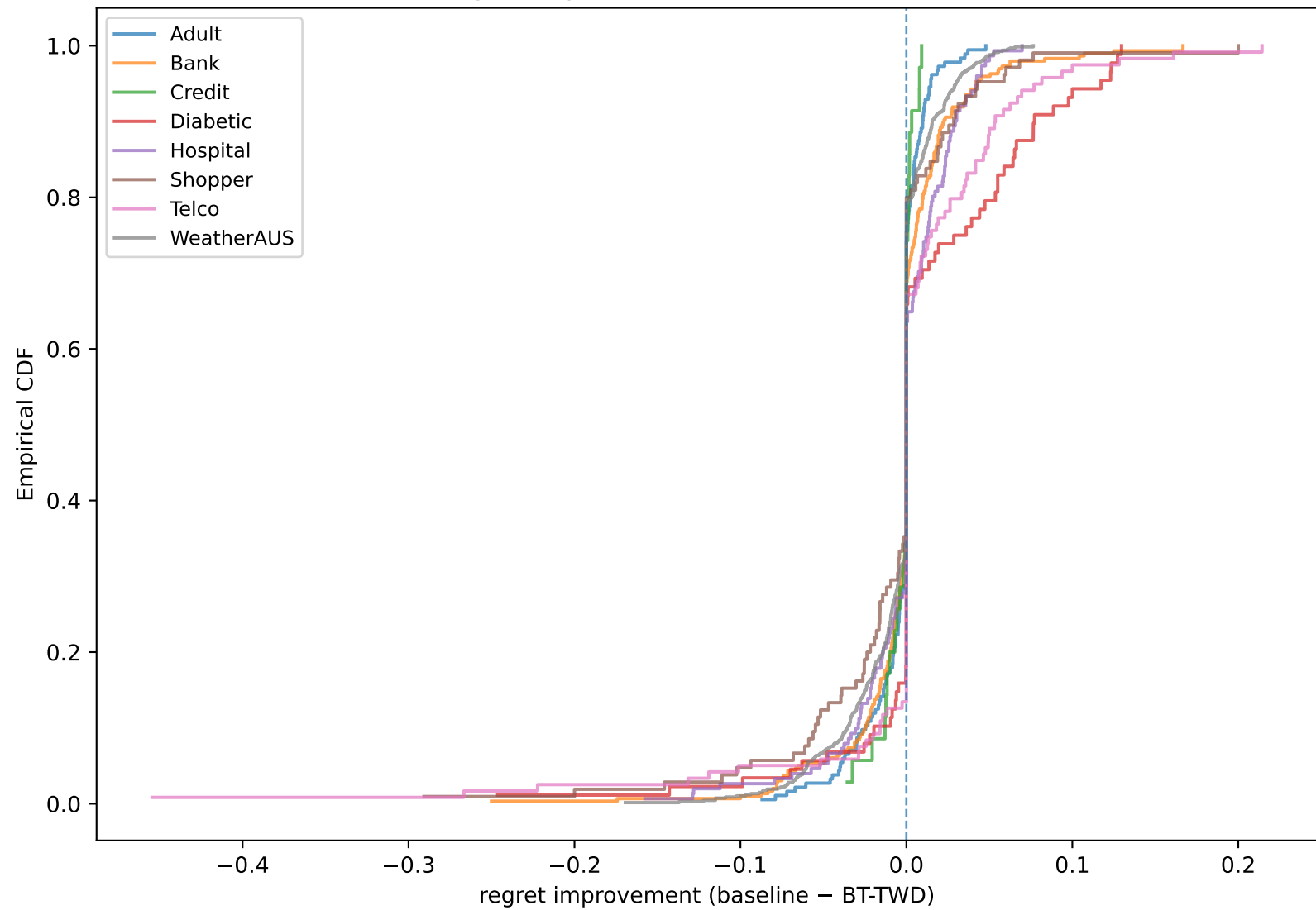
regret improvement (dataset-wise CDF)
