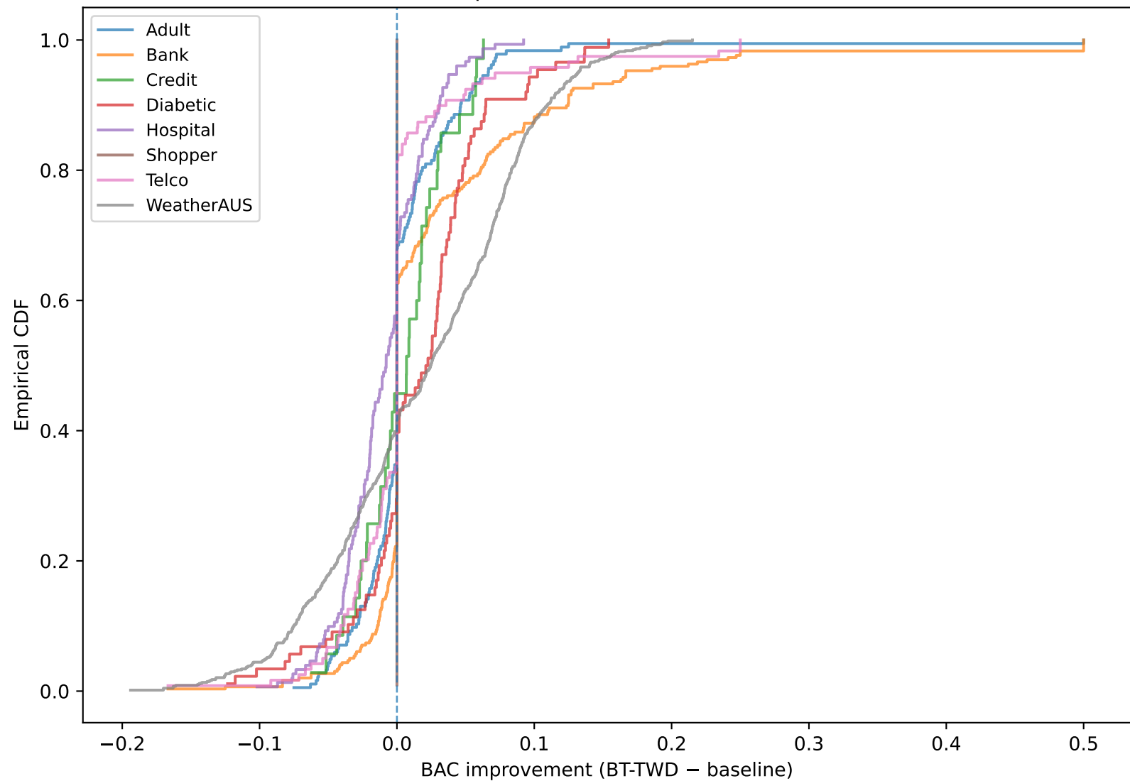
BAC improvement (dataset-wise CDF)
