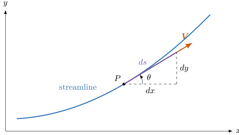
Figure 4: On a streamline, the differential displacement d\mathbf{r} and the local velocity \mathbf{V} are parallel. Thus dy/dx = v/u in two dimensions.
