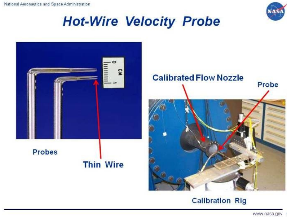
Figure 1: A hot-wire velocity probe measures the air velocity at a fixed location. This is an Eulerian measurement because the instrument remains at one spatial point while fluid particles pass through it. Photo: NASA Glenn Research Center.
