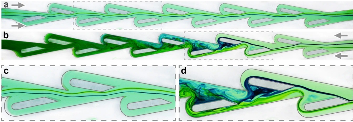
Figure 5: Dye injected continuously upstream forms visible streaklines through a Tesla-valve geometry. The image records many particles that passed through the same injection locations, rather than the complete history of one particle. Photo: Q. M. Nguyen, J. Abouezzi, and L. Ristroph, CC BY 4.0.
