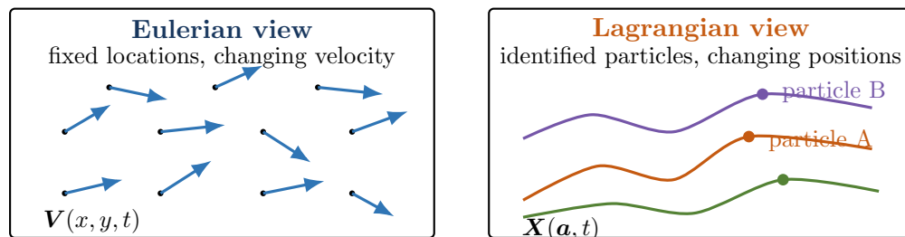
Figure 3: The Eulerian description observes the flow at fixed spatial points; the Lagrangian description follows identified fluid particles.
