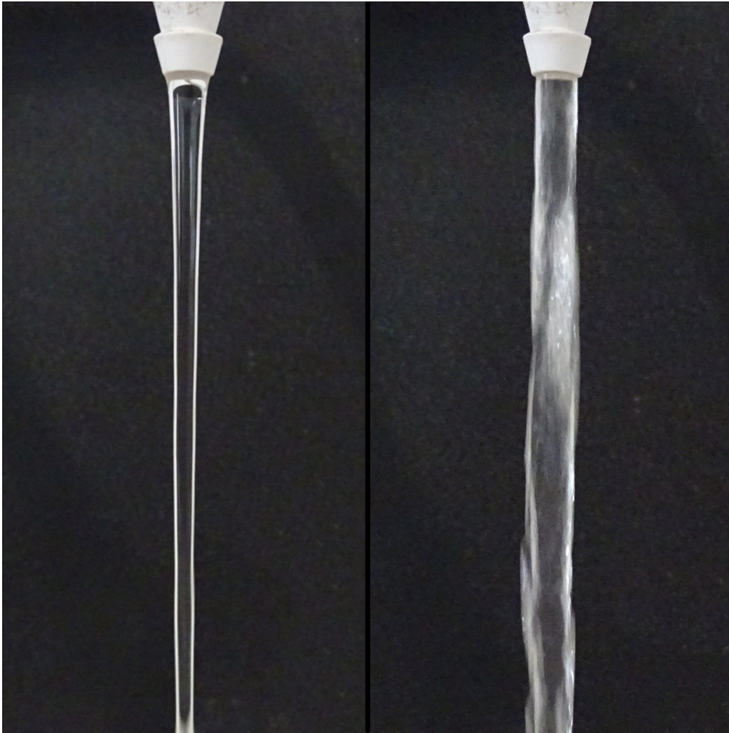
Figure 2: Real water jets showing an orderly laminar jet on the left and an irregular turbulent jet on the right. The turbulent jet contains stronger fluctuations and mixing. Photo: MikeRun, CC BY-SA 4.0.
