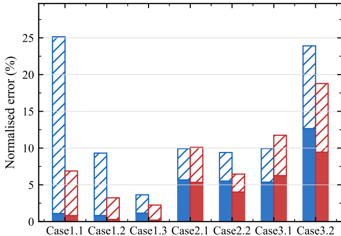
Source term
