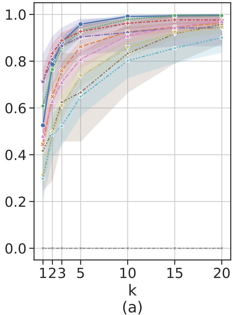
% of Correct Retrieved LoRAs
