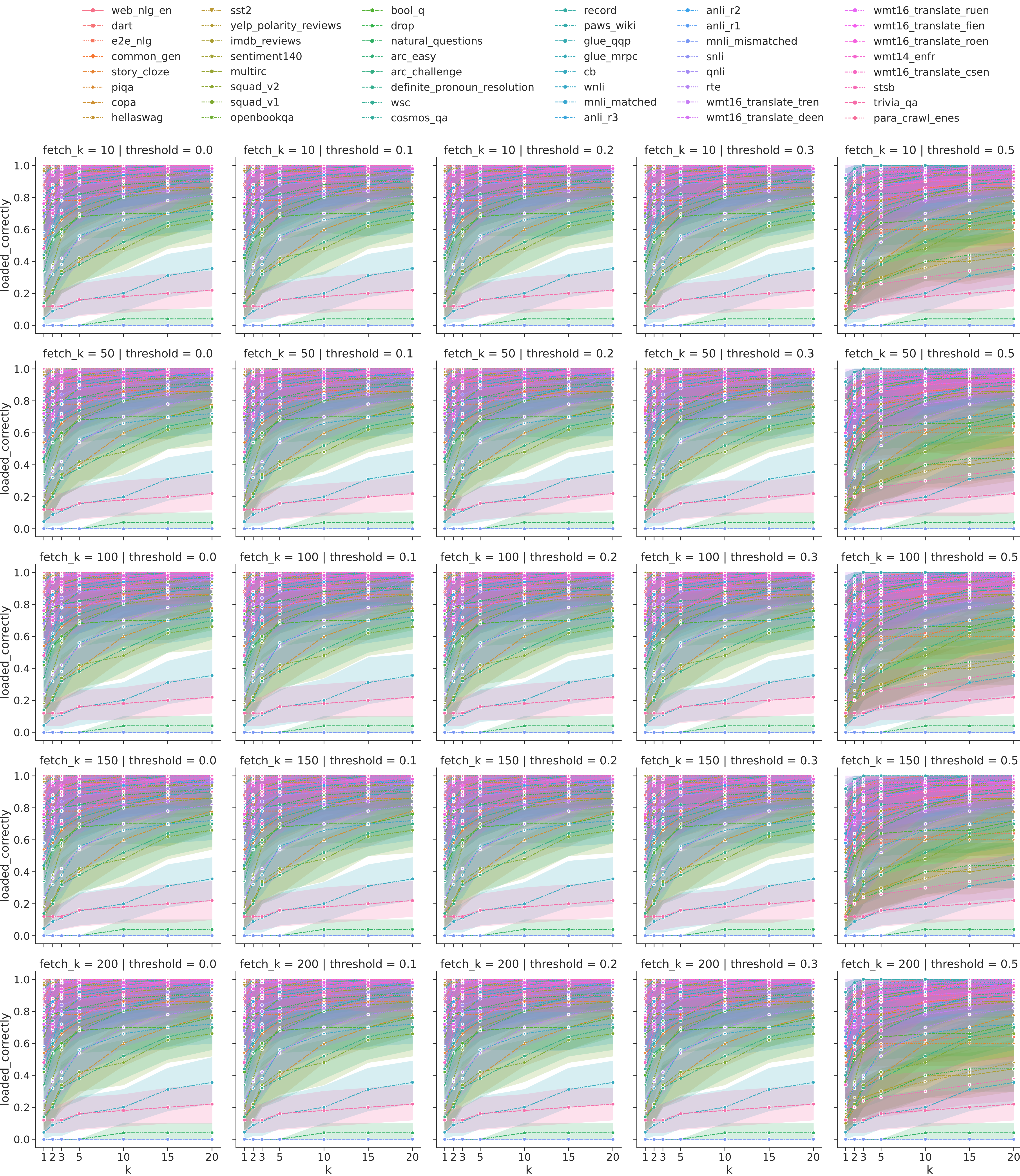
FlanV2 Tasks
