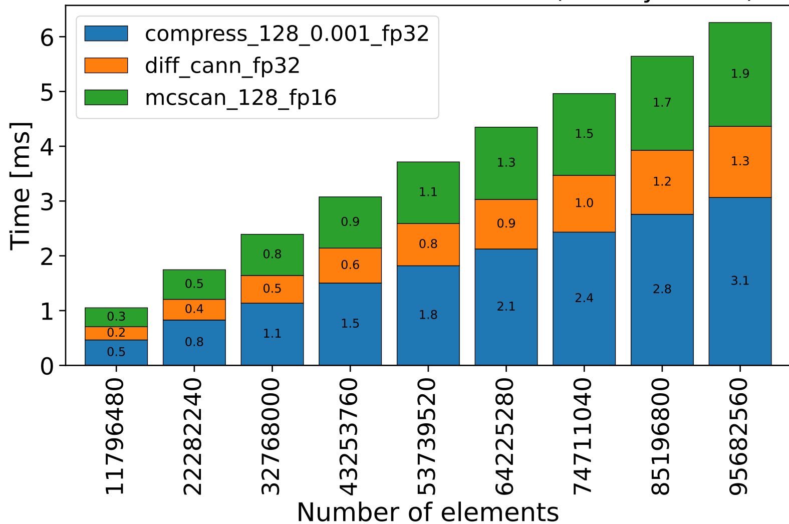
Execution time break-down of SCD (density: 0.001)
